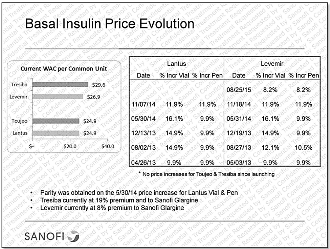
Figure 16: Sanofi price-tracking
