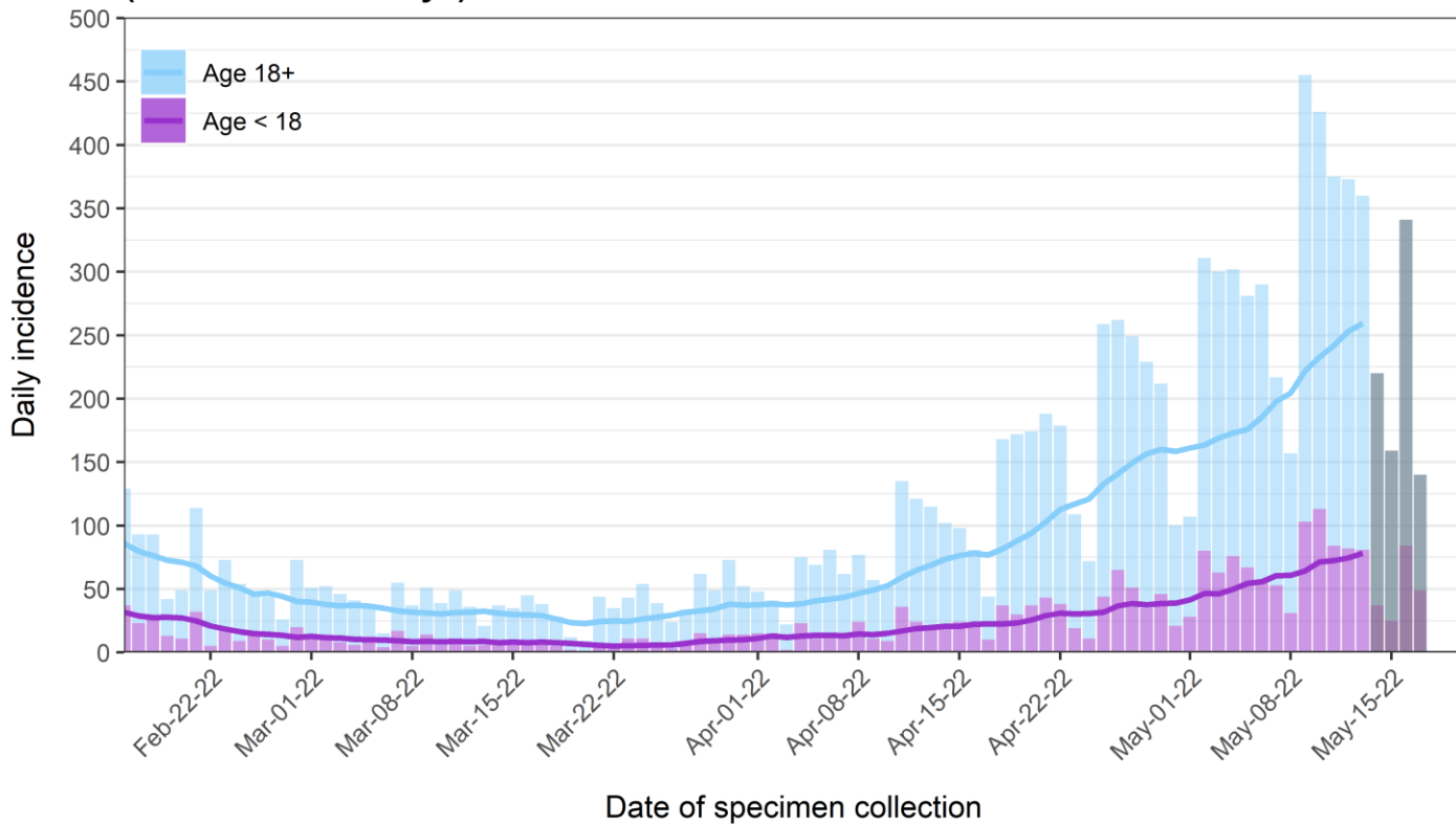
Figure 1b: Stacked bargraph of daily cases in Milwaukee County by age group (most recent 90 days)
